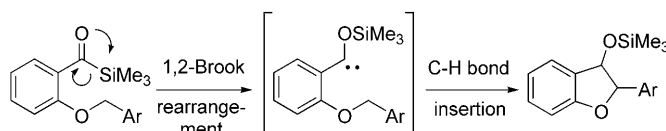
Scheme 1. Proposed mechanism for intramolecular C–H bond functionalization of acylsilanes.
